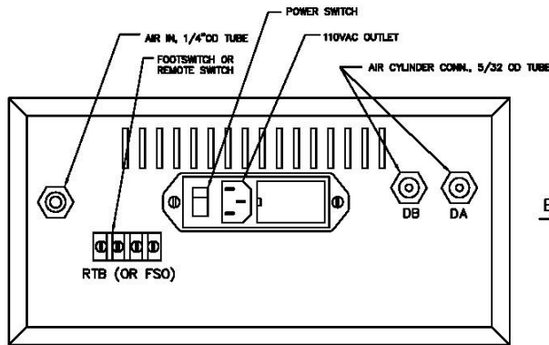
SAC 1000-CONTROLLER FOR P2000 (RELAY TYPE)
